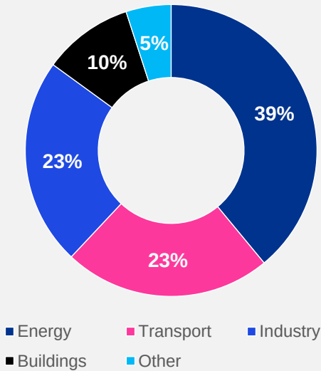
Figure 1: Global CO 2 emissions by sector (as of October 2022) (2)
