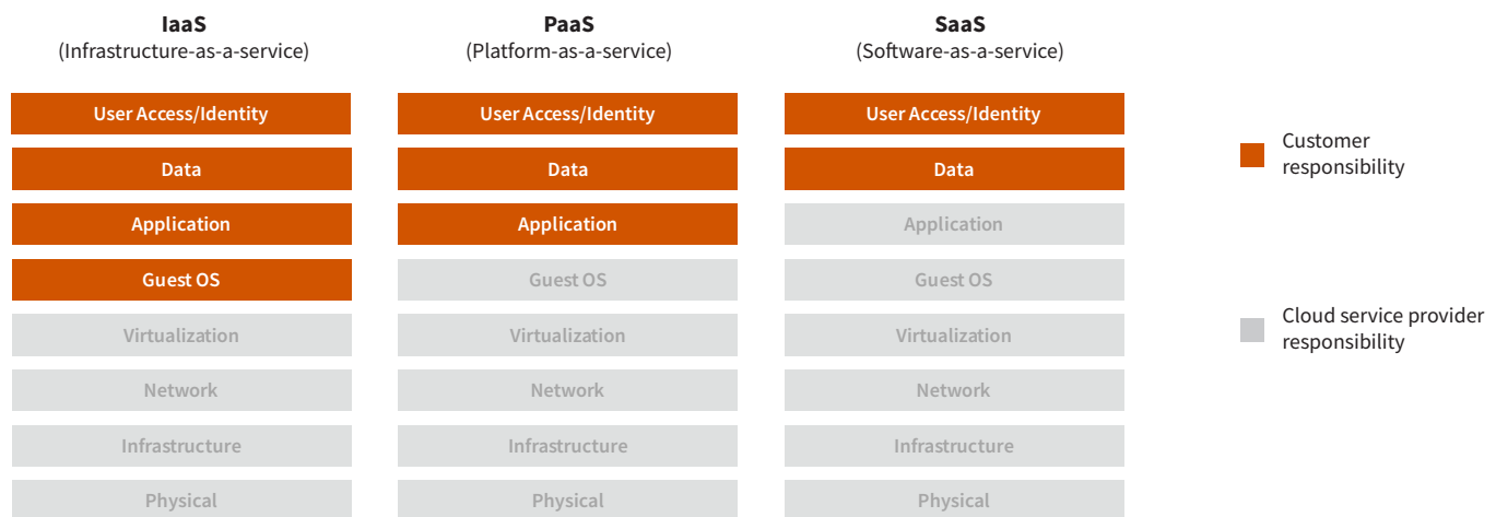
Figure 7. Cloud Security Shared Responsibility Model
